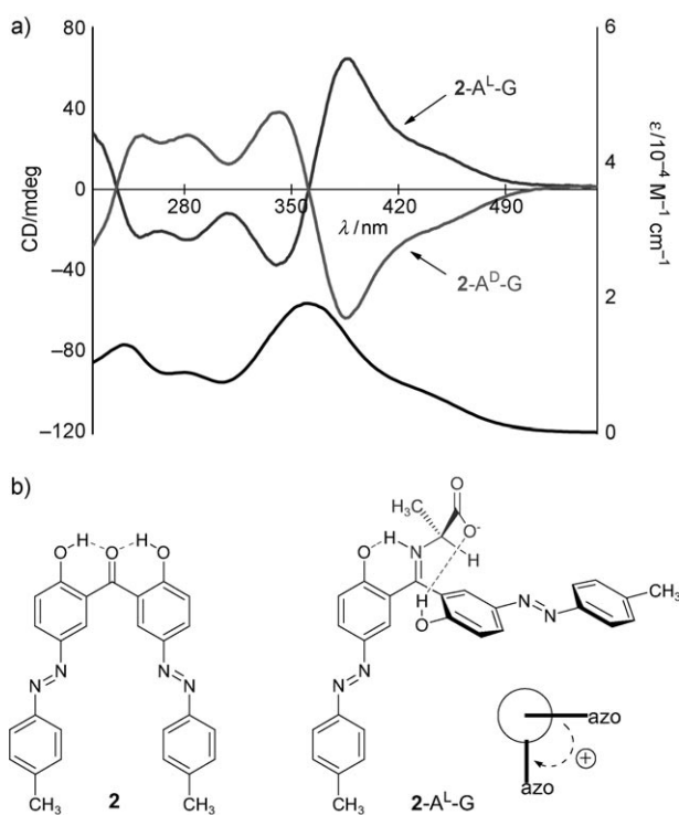
Figure 3. a) Circular dichroism spectra of 2-A L -G and 2-A D -G (50 μm in acetonitrile, 1 cm cell, at 25 °C) and their UV/Vis spectra. b) Structure of 2 and 2-A L -G.
